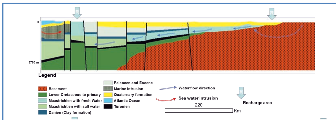
Geological cross-section of the Senegalo-Mauritanian Basin
