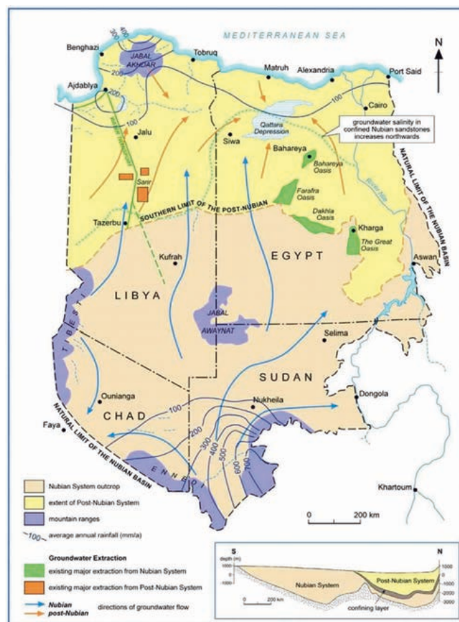
Major groundwater abstraction areas within the Nubian Sandstone Aquifer System
