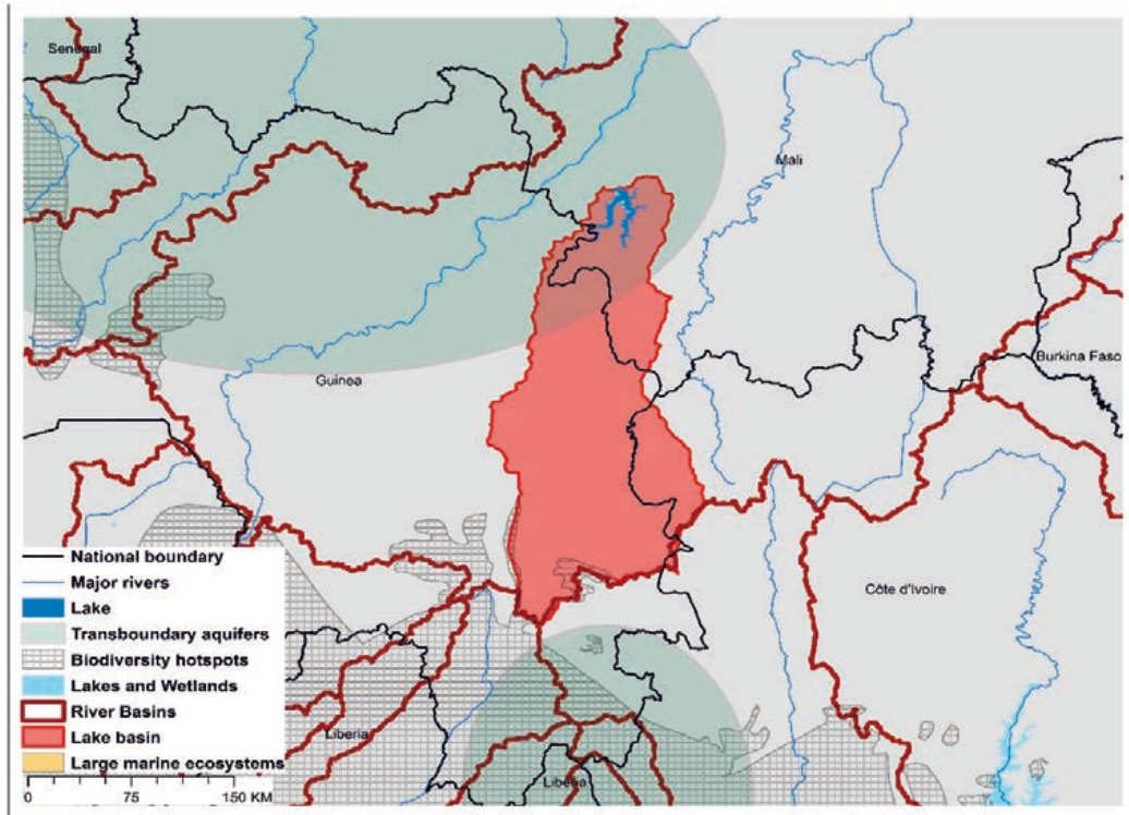
(a) Lake Sélingué basin and associated transboundary water systems
